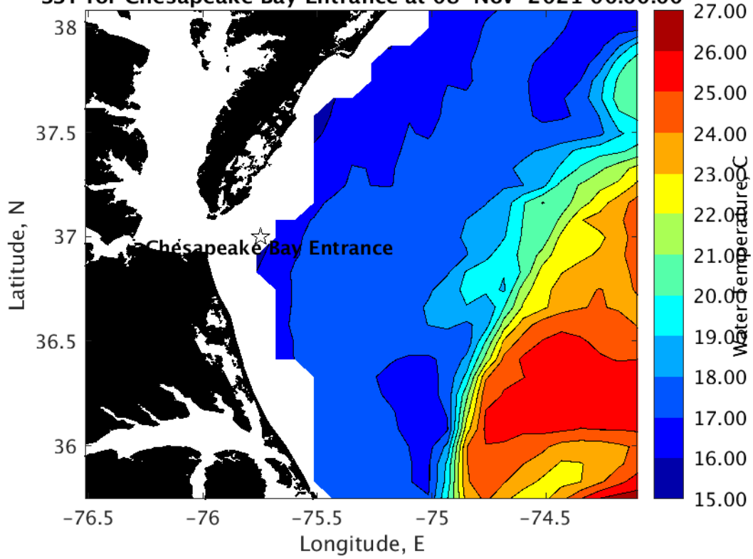
SST for Chesapeake Bay Entrance at 08-Nov-2021 00:00:00
